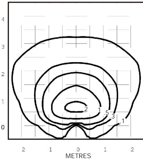
Twig Lite GU4 20 watt Bi-Pin lamp - Lens height 700mm (27½")
