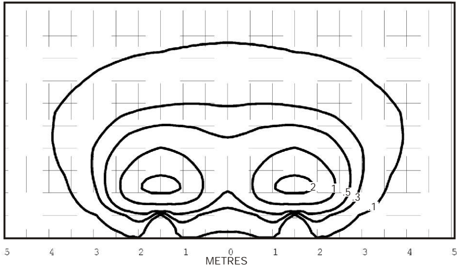
Twig Lite GU4 20 watt Bi-Pin lamp - Lens height 700mm (27½")
