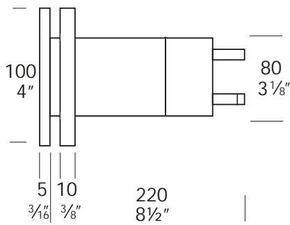
Pool Canister (Supplied with Luminaire)
