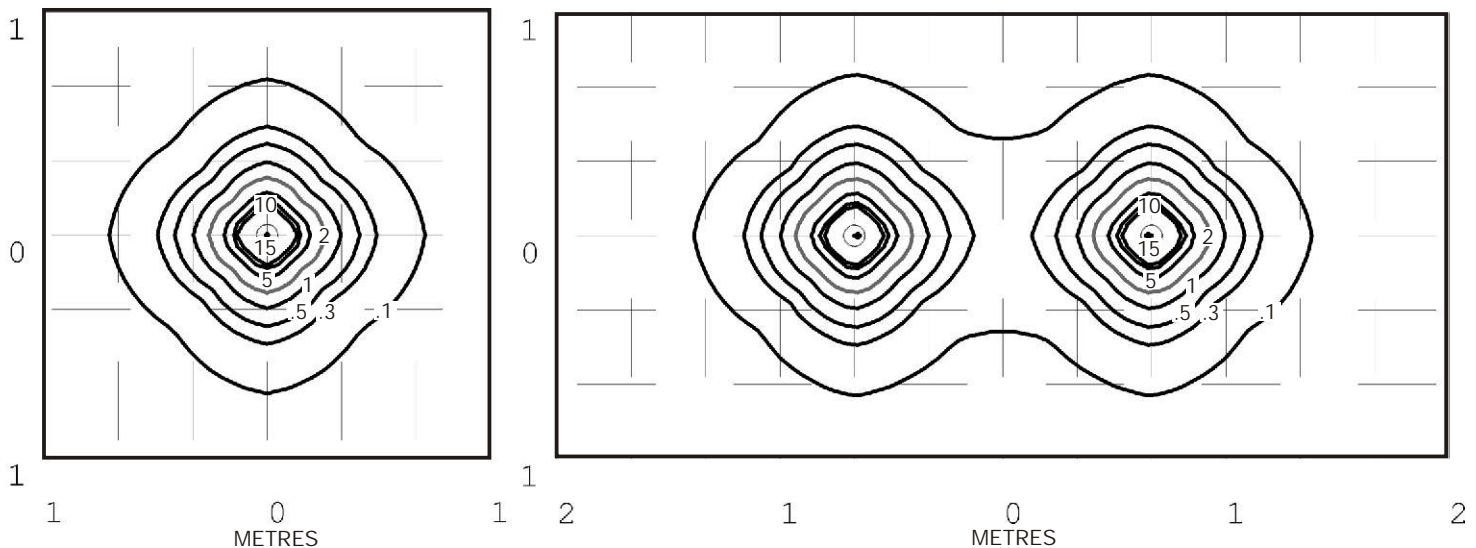
Path Lite 4 facet MR16 ESX 20 watt lamp - Lens height 5mm (¼")
