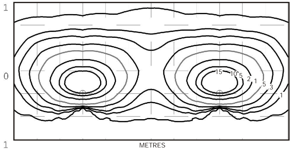
Mouse Lite Square 20 watt GU4 Bi-Pin lamp - Lens height 400mm (15¾")
