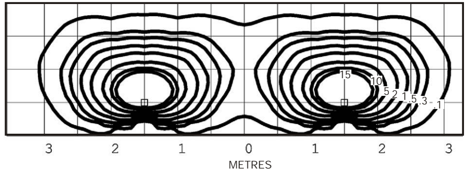
Mouse Lite Square 20 watt GU4 Bi-Pin lamp - Lens height 400mm (15¾")
