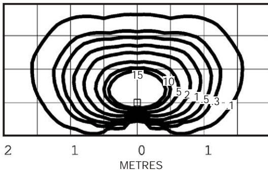
Mouse Lite Square 20 watt GU4 Bi-Pin lamp - Lens height 400mm (15¾")
