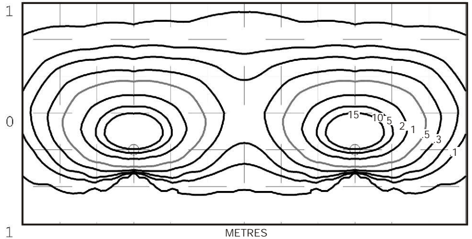
Mouse Lite Square 20 watt GU4 Bi-Pin lamp - Lens height 400mm (15¾")
