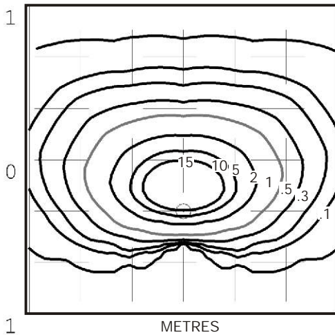
Mouse Lite Square 20 watt GU4 Bi-Pin lamp - Lens height 400mm (15¾")
